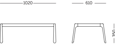
MODULE B - Structure for 2 units
